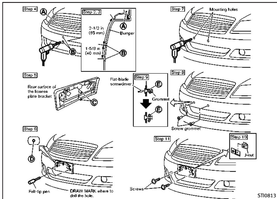
Coupe (except for INFINITI Performance Line model)
