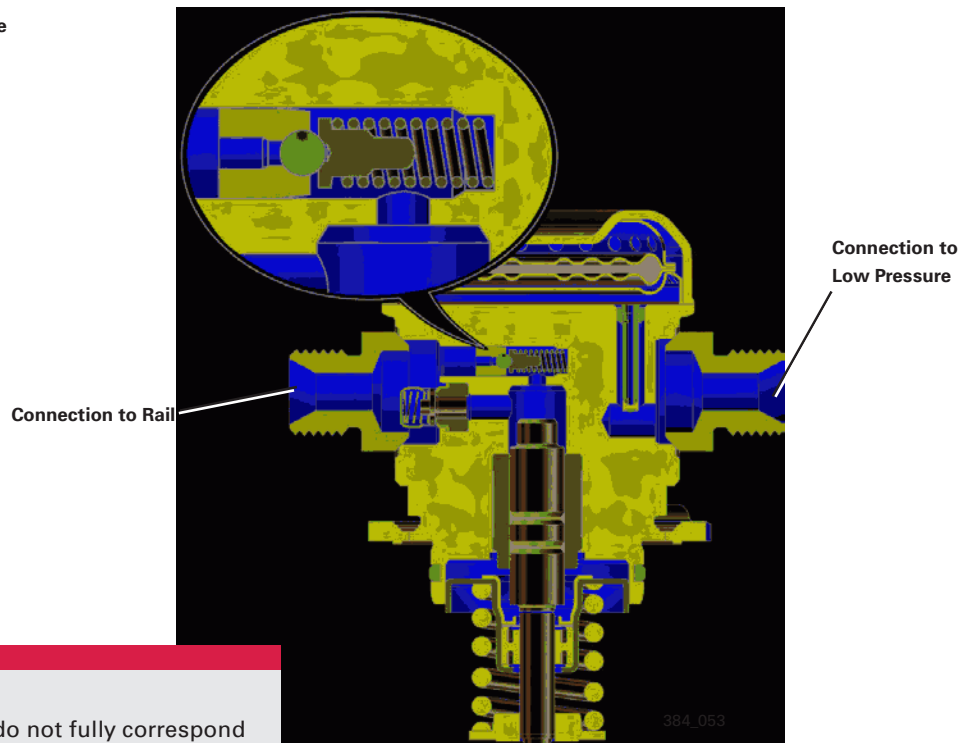
Pressure Limiting Valve
