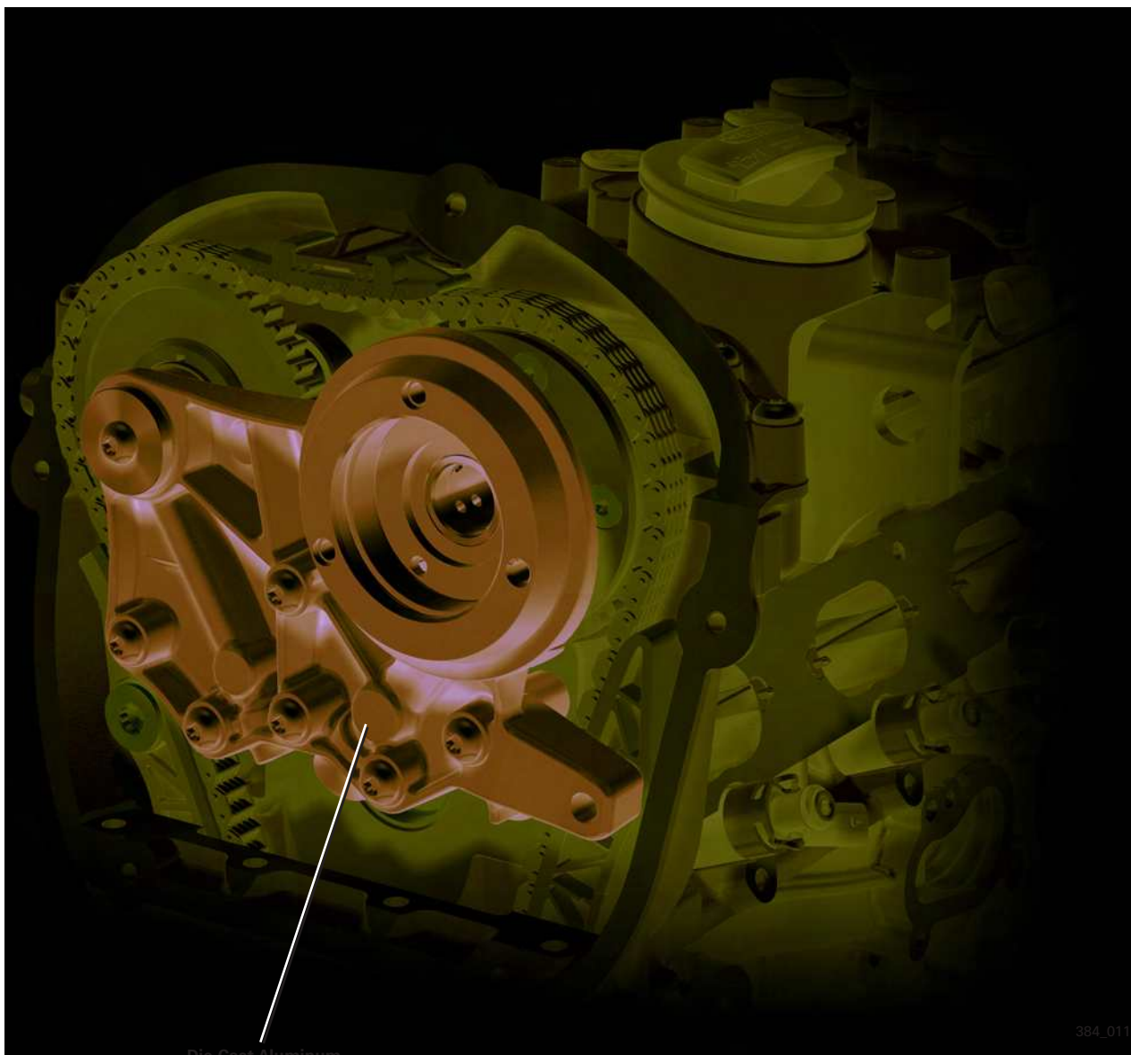
Die-Cast Aluminum Bearing Bridge
