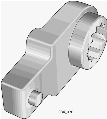
T10360 Torque Wrench Adapter Used for Removing/Installing the Belt Drive Pulley Bolt for the Engine Coolant Pump
