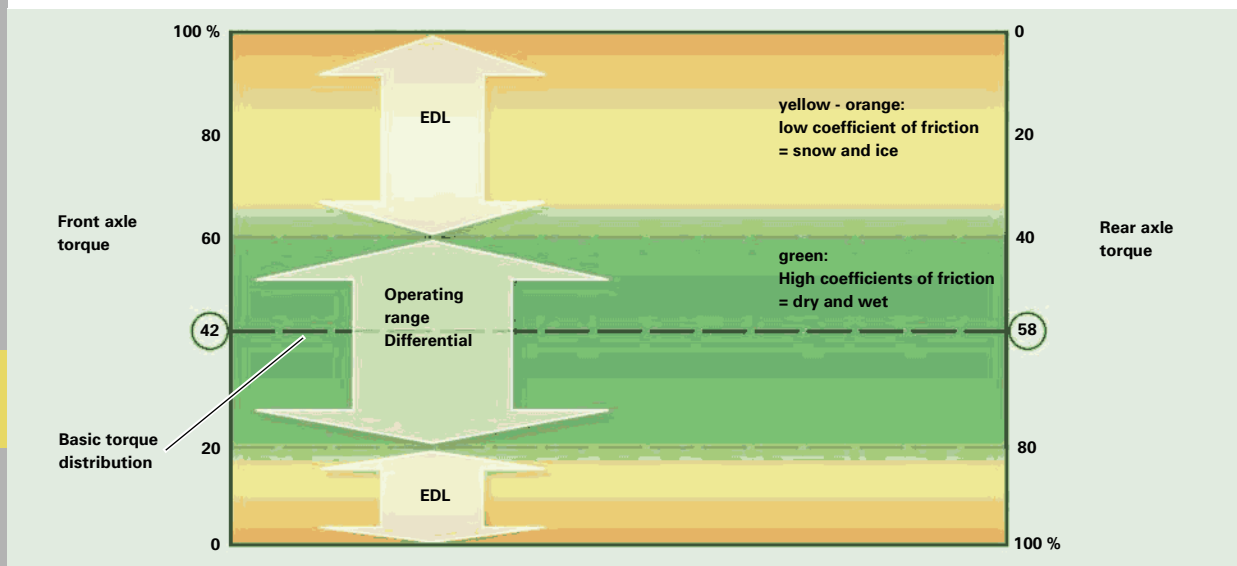
Asymmetric/dynamic torque distribution in the self-locking centre differential (under throttle)
